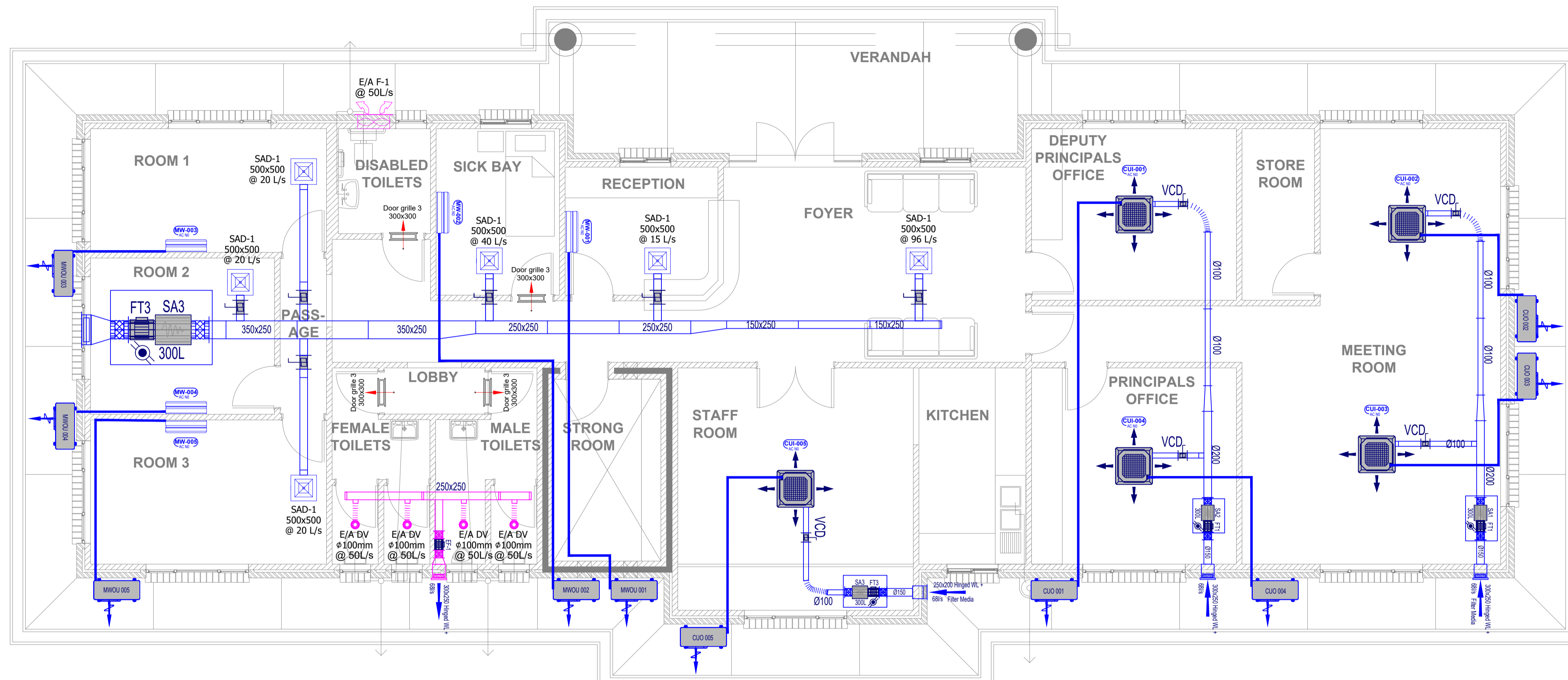
ADMINISTRATION BUILDING SCALE 1:50
